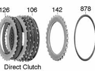
Direct Clutch
